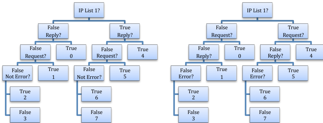
Figure 2. Diagrams for icmp.tree. Left: source tree; right: destination tree. ICMP types 8, 10, 13, 15, and 17 correspond to requests; 0, 9, 14, 16, and 18 correspond to replies, and types 3, 4, 5, 11, and 12 correspond to errors.
